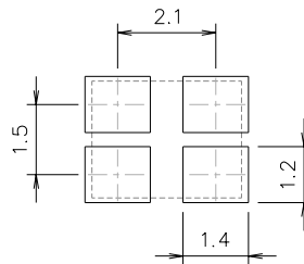
Reference Footprint
